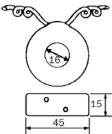
Foot mounting option (F)
